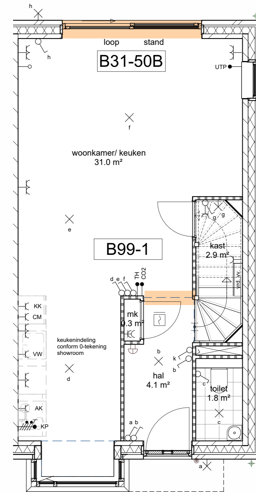
G3/G3s - begane grond
