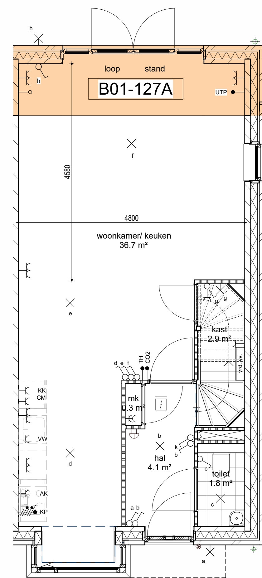
G3/G3s - begane grond
